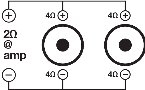
WIRED IN PARALLEL TO A 1-OHM OR 2-OHM STABLE MONO AMPLIFIER
